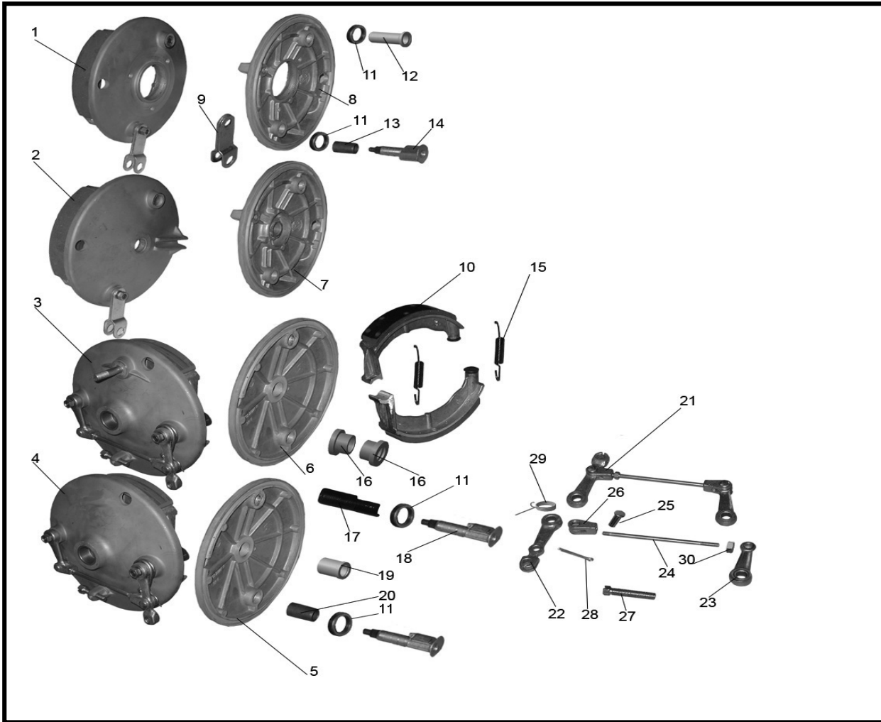
Figure 41. - Brake Drum and Components
